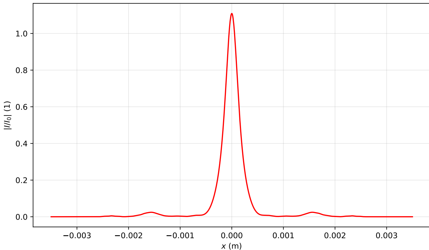
Intensity profile I(x, y = 0, z = 0.955)/I_0 , P_{in}=5.0P_{cr} , artificial time
